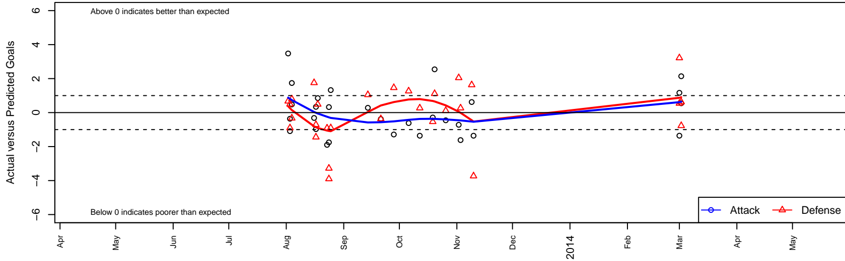
CB United Navy B01 Dots are actual minus expected GF (blue circles) and GA (red triangles). Blue line is smoothed change in attack strength. Red is smoothed change in defense strength.
